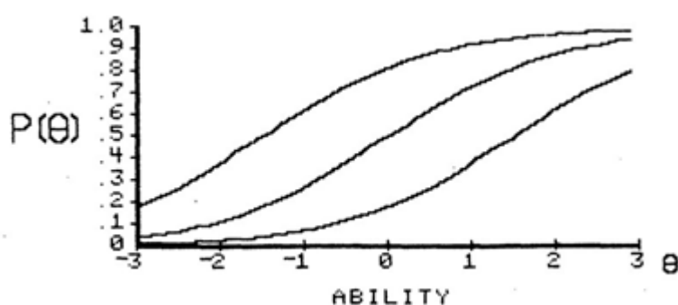
Figure 3: Three item characteristic curves with the same discrimination but different levels of difficulty (Baker, 2001, p. 10)
